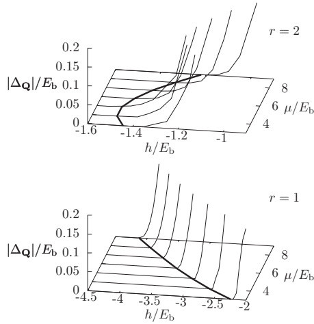
FIG. 3. Variation of the order parameter |\Delta_{\mathbf{Q}}|/E_b with chemical potential difference h/E_b and chemical potential \mu/E_b . The upper panel is at a mass ratio r=2 , and the lower panel at equal masses, r=1 . The thin black lines trace out the |\Delta_{\mathbf{Q}}|/E_b variation, found by minimizing the thermodynamic potential (1), for several different chemical potentials. The thick black line is the locus of the second-order transition predicted by Ginzburg-Landau theory.
